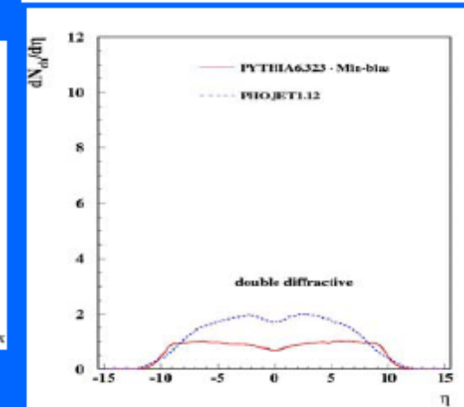
Double diffractive DD
