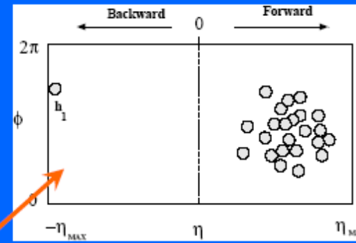
Single diffractive SD
