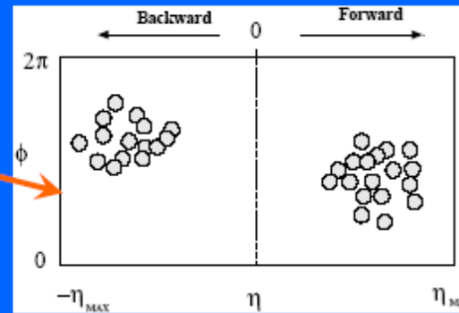
Double diffractive DD
