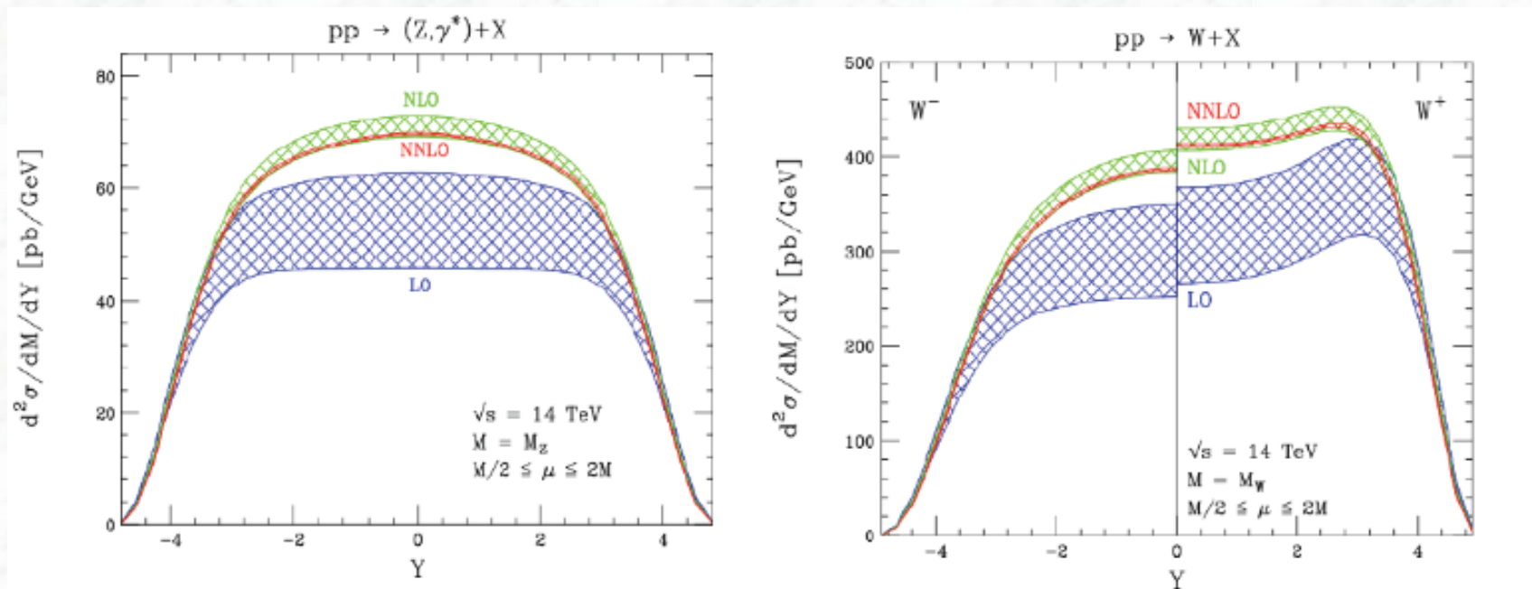
Rapidity distributions for Z and W^\pm production at LO, NLO, and NNLO
