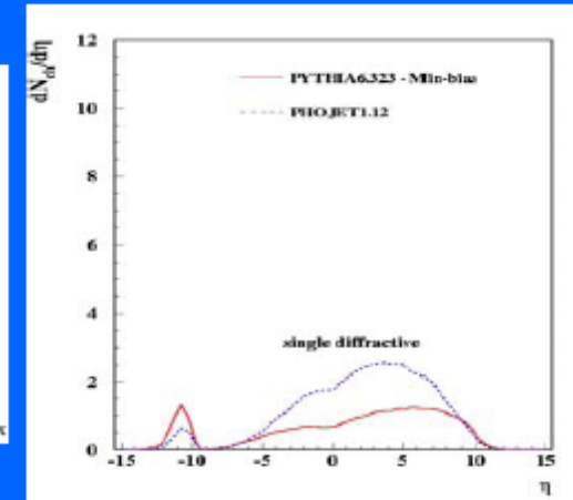
Single diffractive SD
