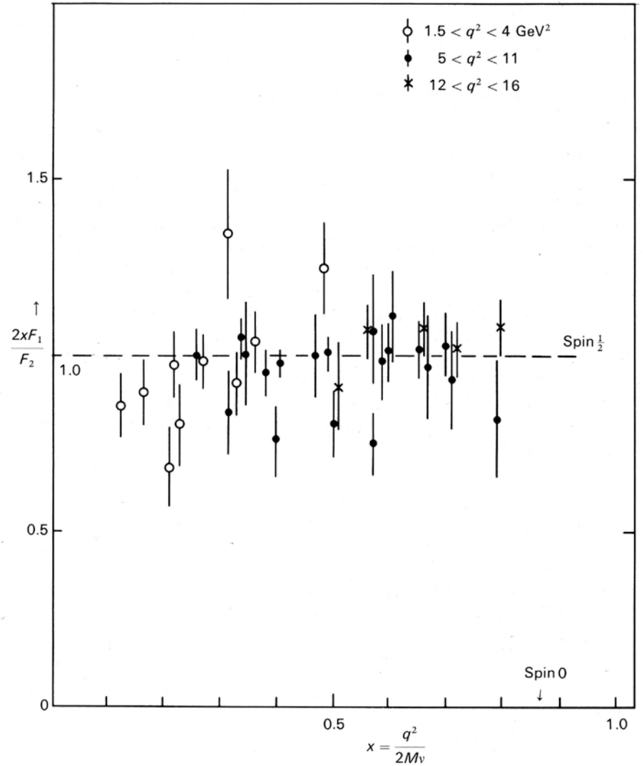
The ratio 2xF_1/F_2 measured in SLAC electron-nucleon scattering experiments. For spin- \frac{1}{2} partons, with g = 2 , a ratio of unity is expected in the limit of large q^2 – the Callan-Gross relation. (Data compiled from published SLAC data.)
