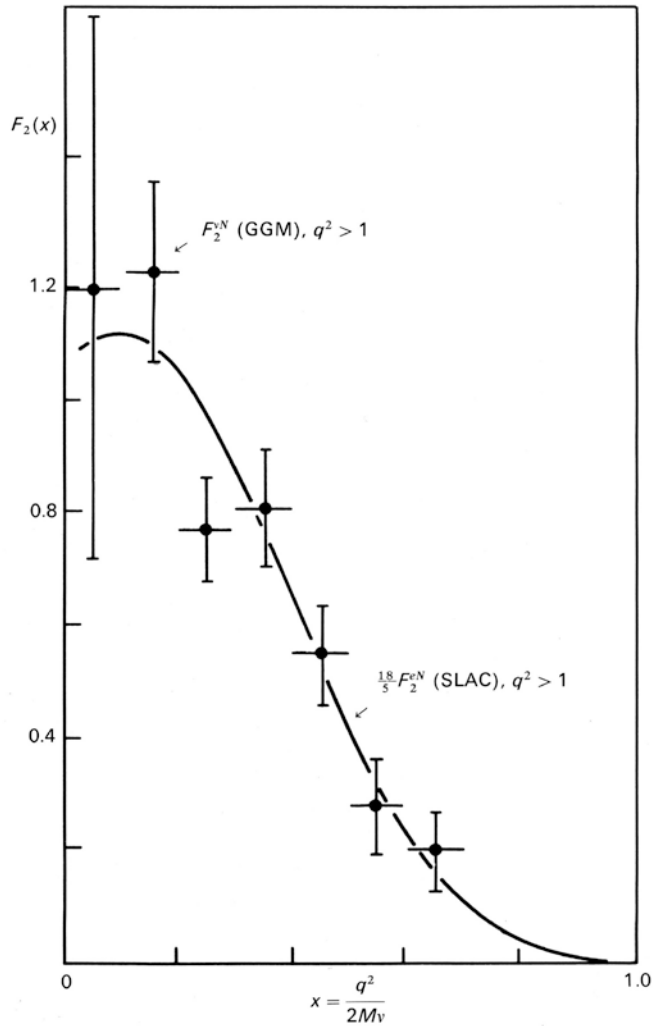
Comparison of F_2^{vN} measured in neutrino-nucleon scattering in the Gargamelle heavy-liquid bubble chamber in a PS neutrino beam at CERN, with SLAC data on F_2^{eN} from electron-nucleon scattering, in the same region of q^2 . The data points are the neutrino results, and the curve is a fit through the electron data, multiplied by the factor \frac{18}{5} , which is the reciprocal of the mean squared charge of u - and d -quarks in the nucleon. This is a confirmation of the fractional charge assignments for the quarks. Note that the total area under the curve, measuring the total momentum fraction in the nucleon carried by quarks, is about 0.5. The remaining mass is ascribed to gluon constituents, which are the postulated carriers of the interquark color field
