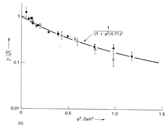
Comparison of the magnetic and electric form factors of neutron and proton. They are consistent with the scaling law (7.34). (a) Proton magnetic form factor; (b) proton electric form factor; (c) neutron magnetic form factor. (After Weber 1967.)
